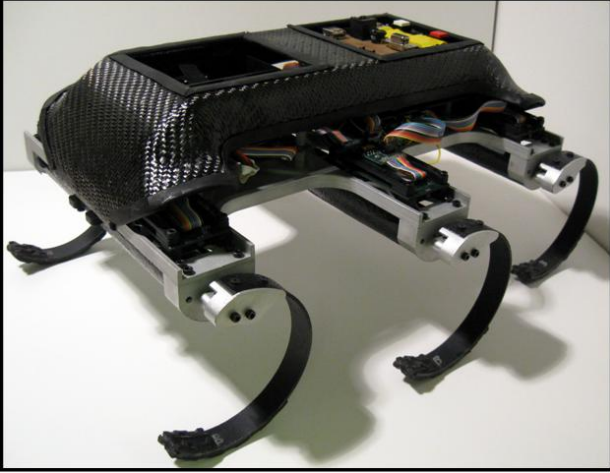
Figure 1. EDUBOT, A HEXAPEDAL DYNAMIC LEGGED LOCOMOTION PLATFORM [6].
